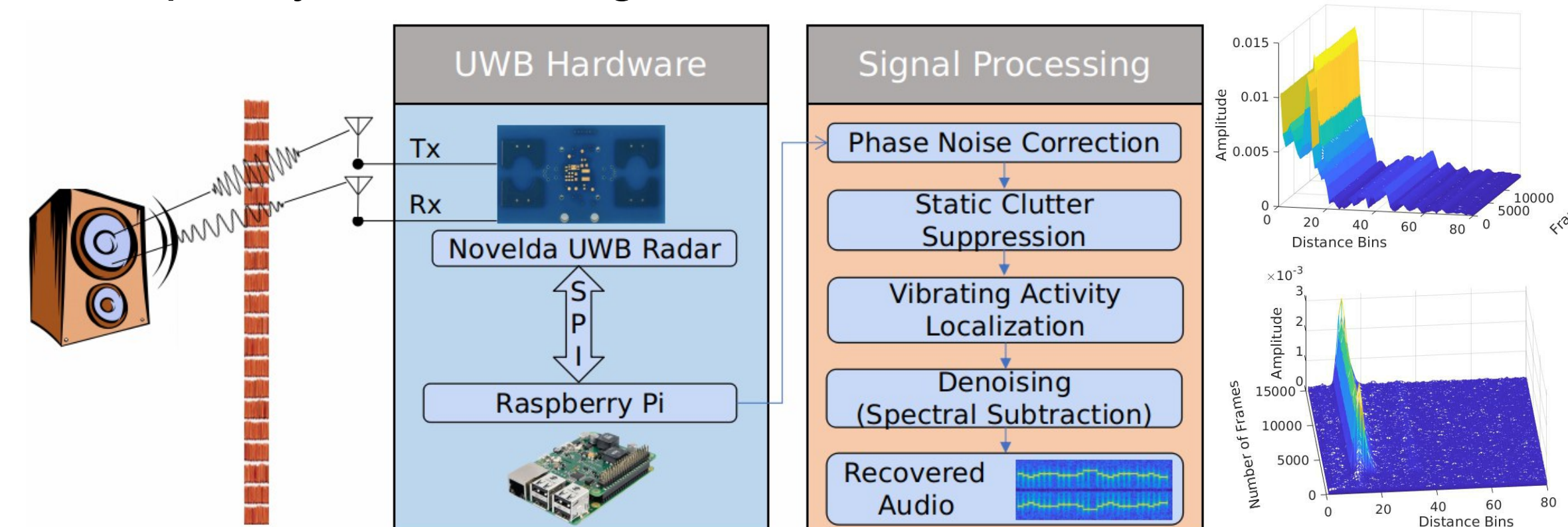
(Left)System overview. (Right Top) 3D visualization of UWHear raw data. (Right Bottom) 3D visualization of UWHear data after processing.
